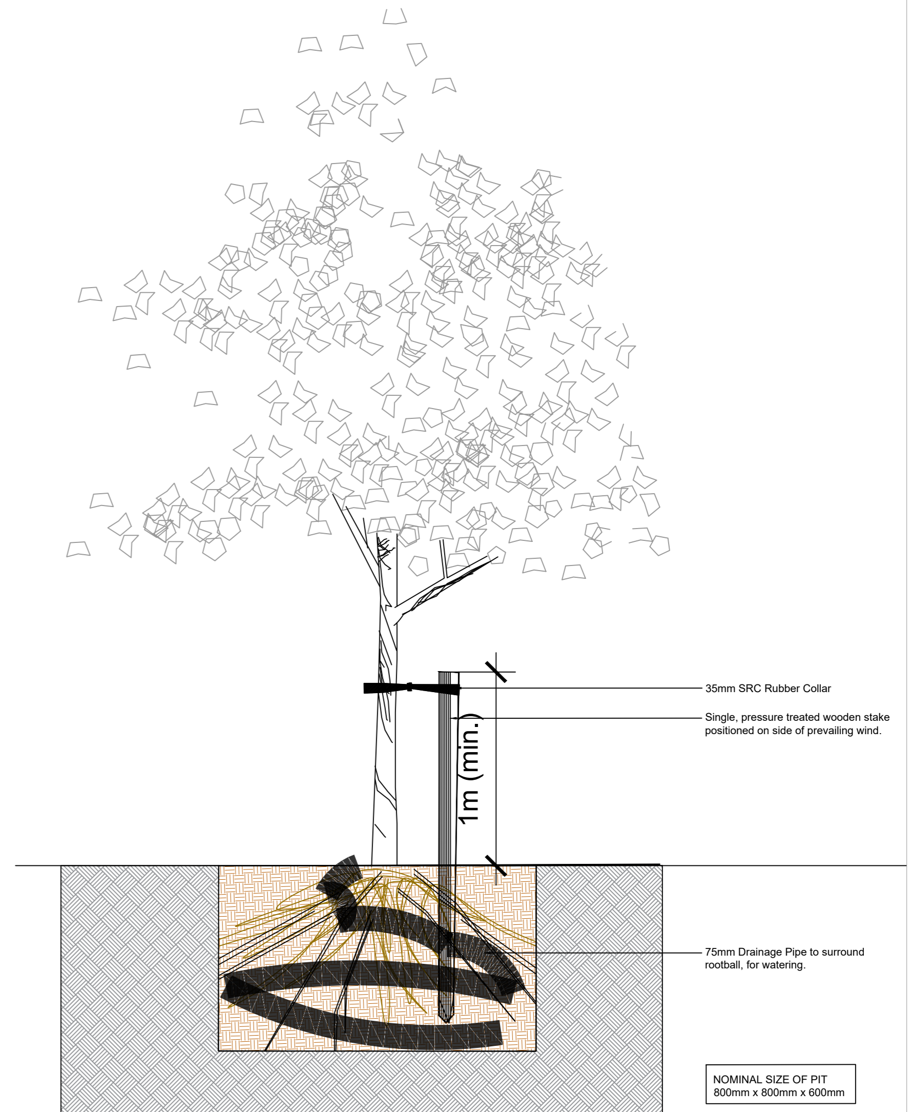
D2 Tree Planting Detail - Single Staking Standard Tree less than 14cm girth Scale 1:20
