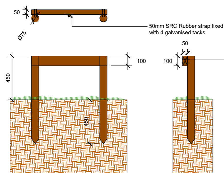
D6 Staking Detail Scale 1:20
