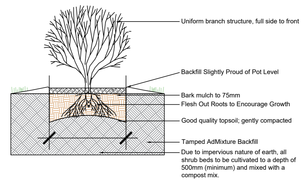
D7 Shrub Planting Detail Scale 1:20
