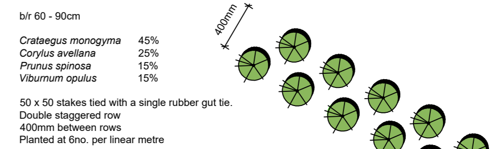
D3 Native Hedgerow Planting Mix - H1 Scale 1:5
